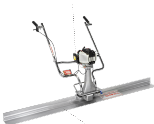
PROFILO - PROFILE
